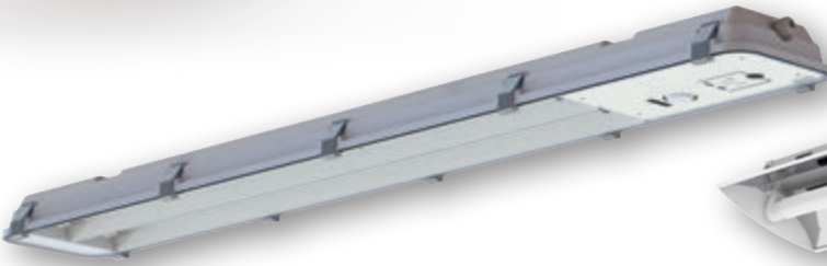
UV-C IP65 Waterproof Disinfection Luminaire
