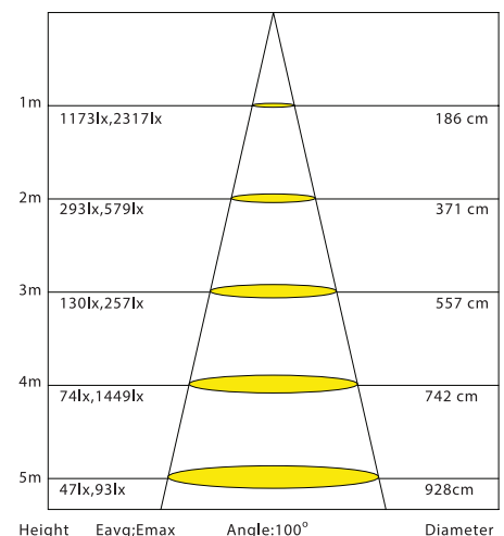
Conic Diagram - 5612 6161
