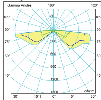
90° Wing Angle (6th level) Light Distribution Curve
