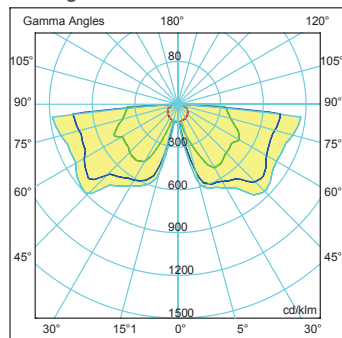
45° Wing Angle (3rd level) Light Distribution Curve
