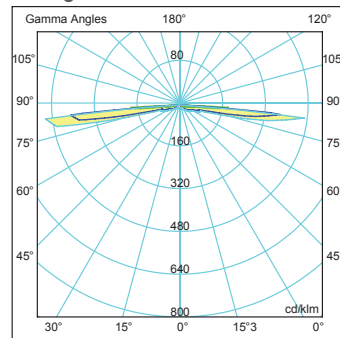
105° Wing Angle (7th level) Light Distribution Curve
