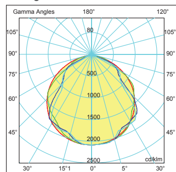
0° Wing Angle Light Distribution Curve
